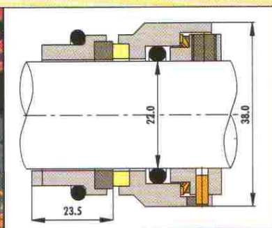
Photo illustrates Type 1690, Type 1689 has straight outer rotary profile.
